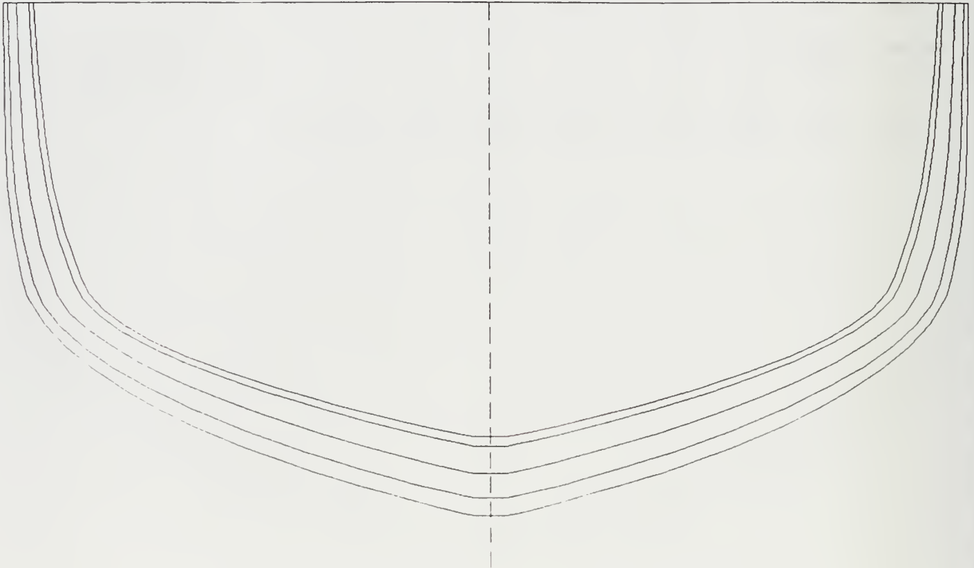
COMP_I.C Body Plan (1 component) Scale = 1:100
